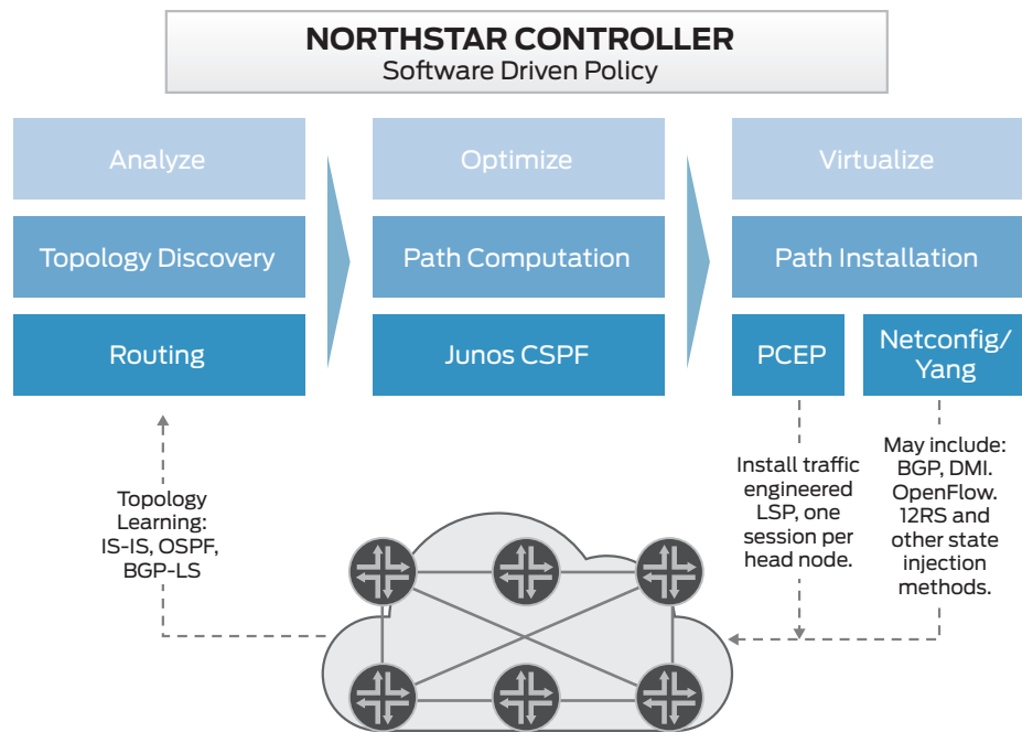
Figure 4. Typical NorthStar Controller workflow
