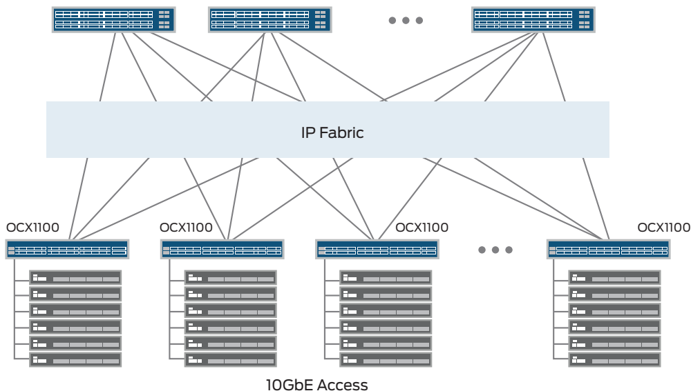
Figure 1: IP fabric deployment using the OCX1100
