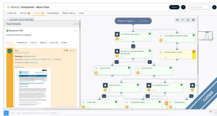
Figure 4: Intelligence-based automated playbook
